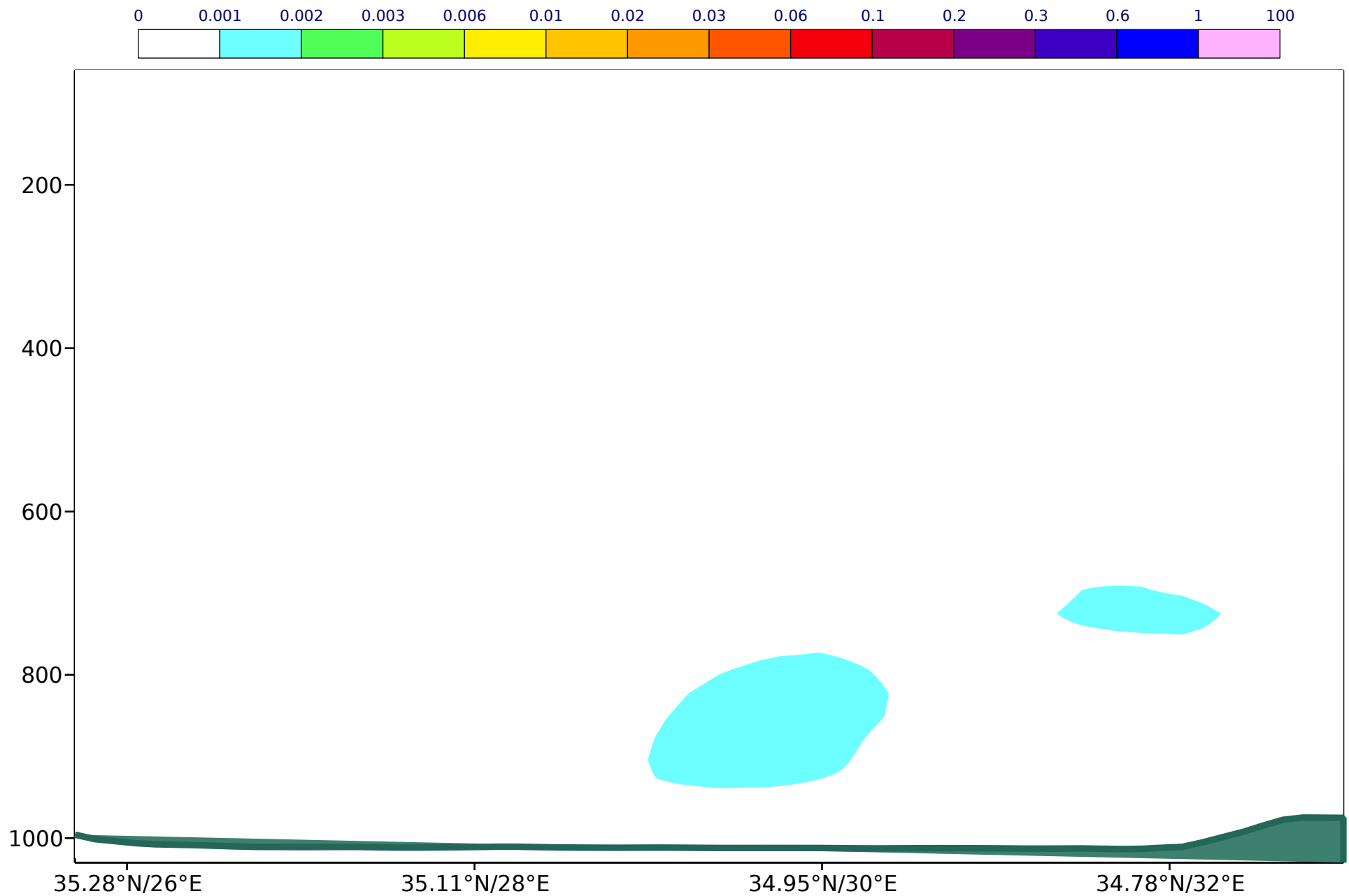
CAMS forecast from Tuesday 18 April 2017 00Z valid at T+000: Tuesday 18 April 2017 00Z Vertical cross-section of Hydrophobic Black Carbon Aerosol Concentration (mg/m 3 ) from (35.3°N,25.7°E) to (34.7°N,33°E)
