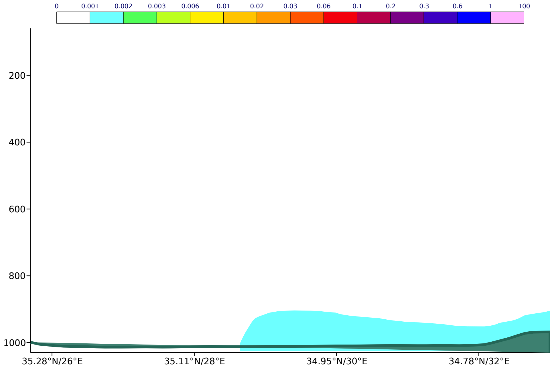
CAMS forecast from Sunday 23 April 2017 00Z valid at T+000: Sunday 23 April 2017 00Z Vertical cross-section of Hydrophobic Black Carbon Aerosol Concentration (mg/m 3 ) from (35.3°N,25.7°E) to (34.7°N,33°E)
